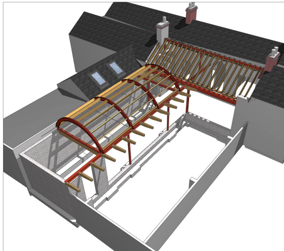
5 TIMBER ROOF STRUCTURES
